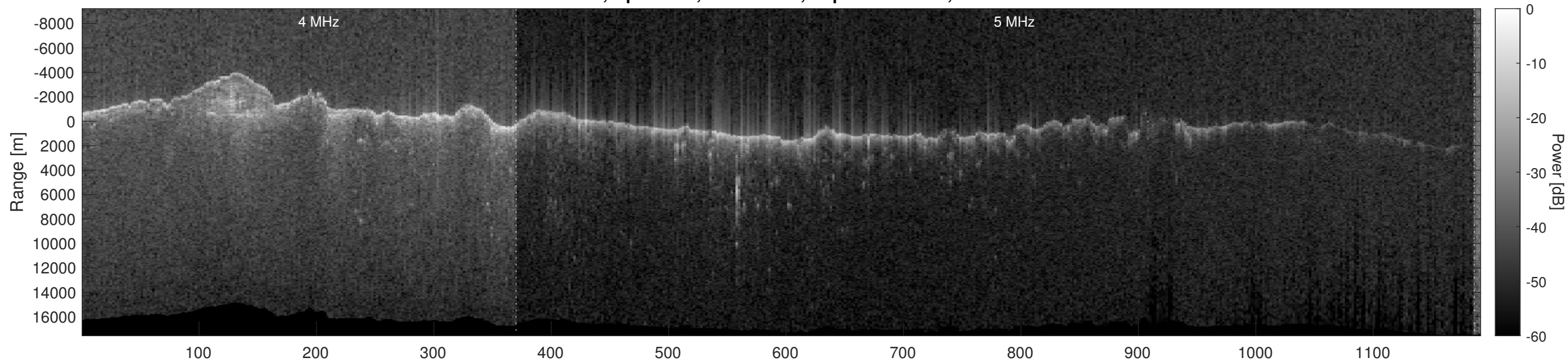
Orbit 8493, Optimized, No Window, Depth-Corrected, Channel 2
