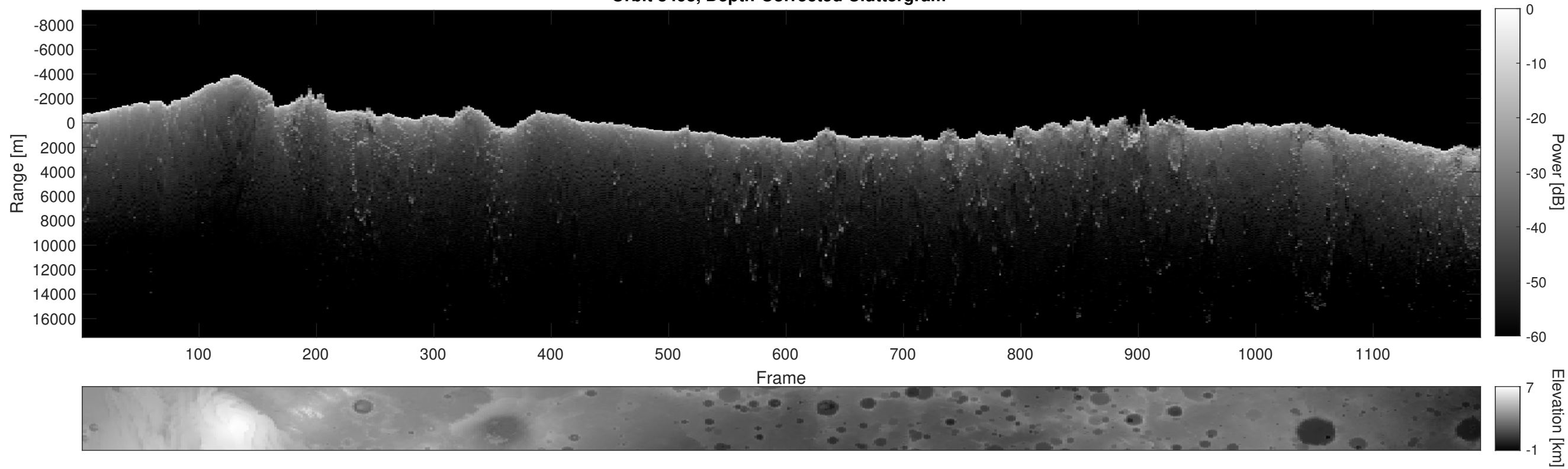
Orbit 8493, Depth-Corrected Cluttergram
