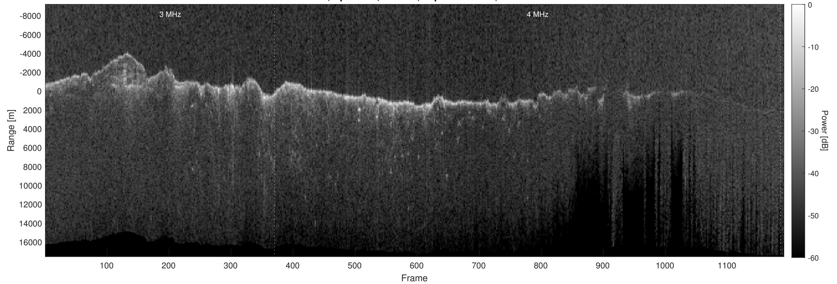
Orbit 8493, Optimized, Window, Depth-Corrected, Channel 2
