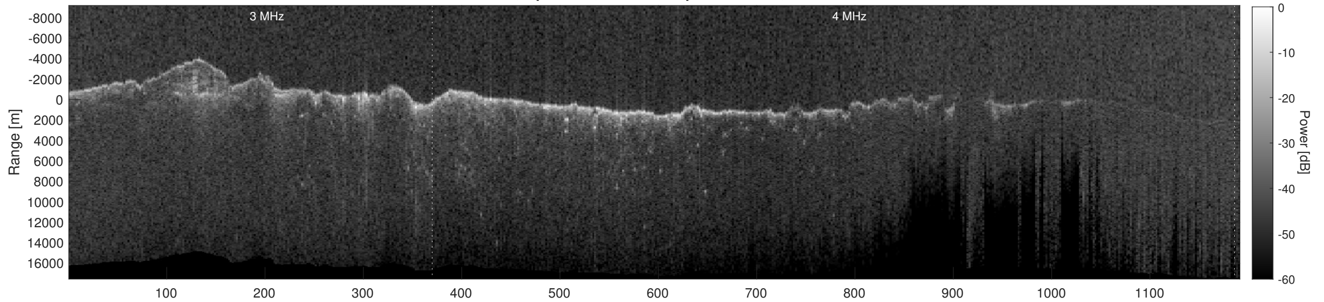
Orbit 8493, Depth-Corrected Cluttergram
