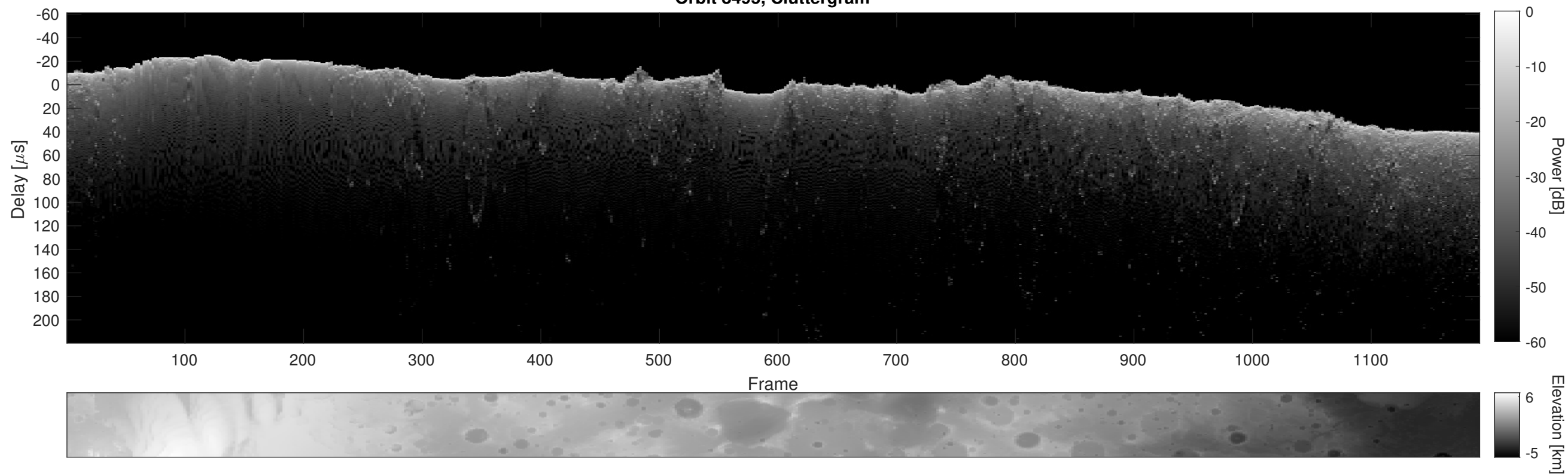
Orbit 8495, Cluttergram
