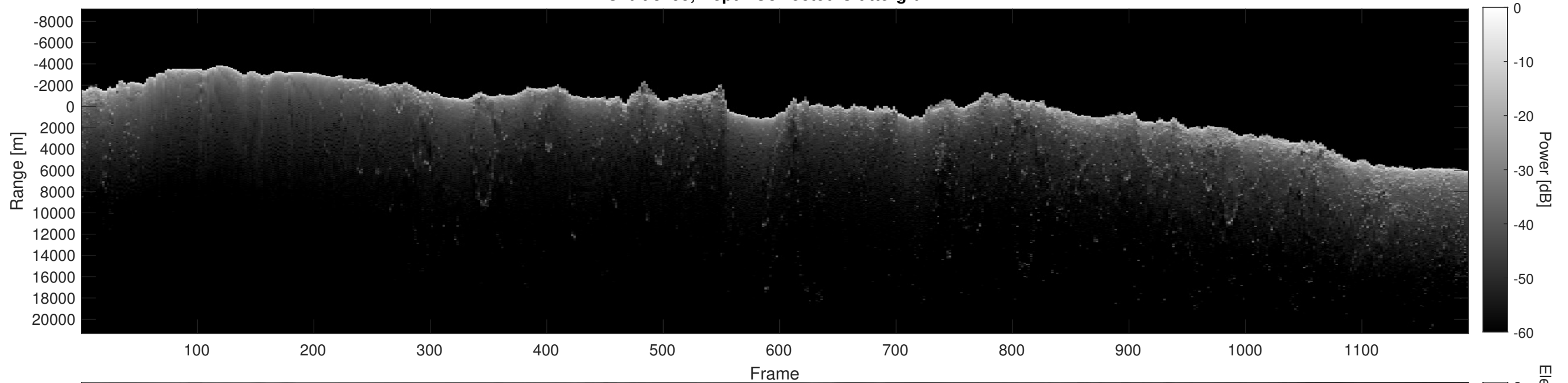
Orbit 8495, Depth-Corrected Cluttergram
