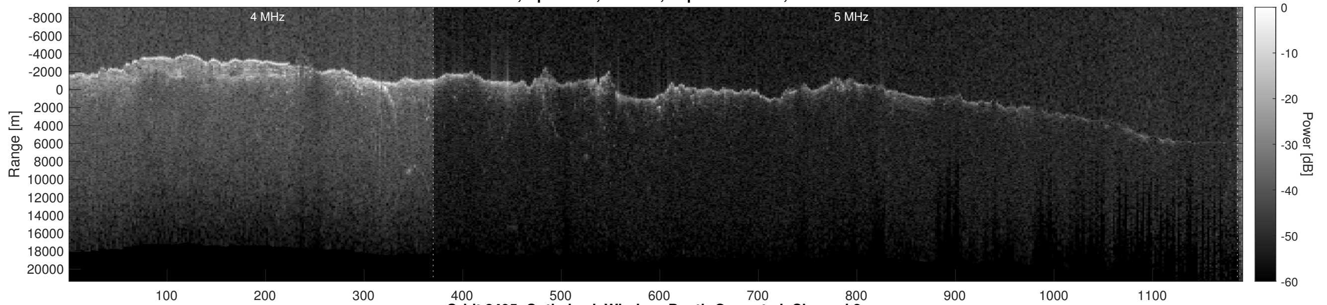
Orbit 8495, Optimized, Window, Depth-Corrected, Channel 2
