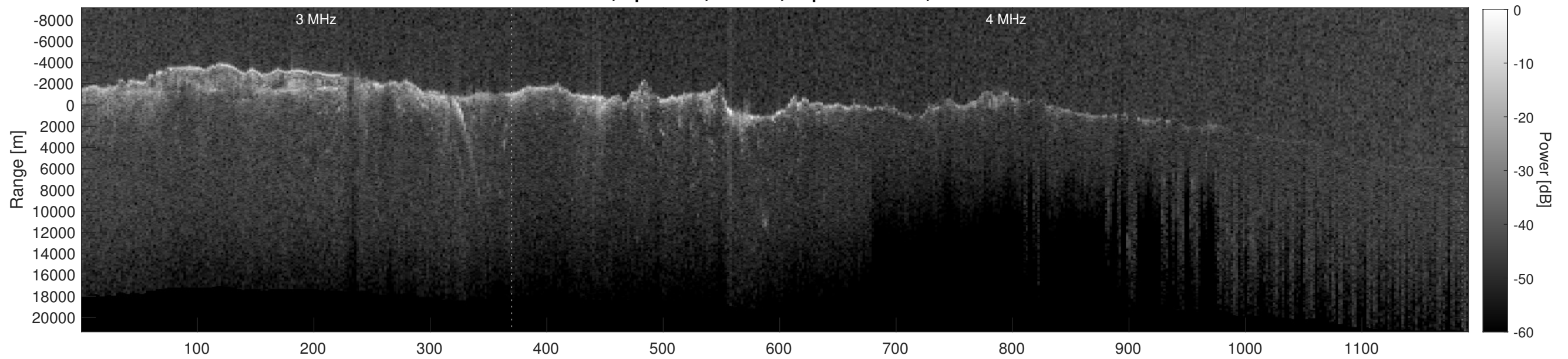
Orbit 8495, Depth-Corrected Cluttergram
