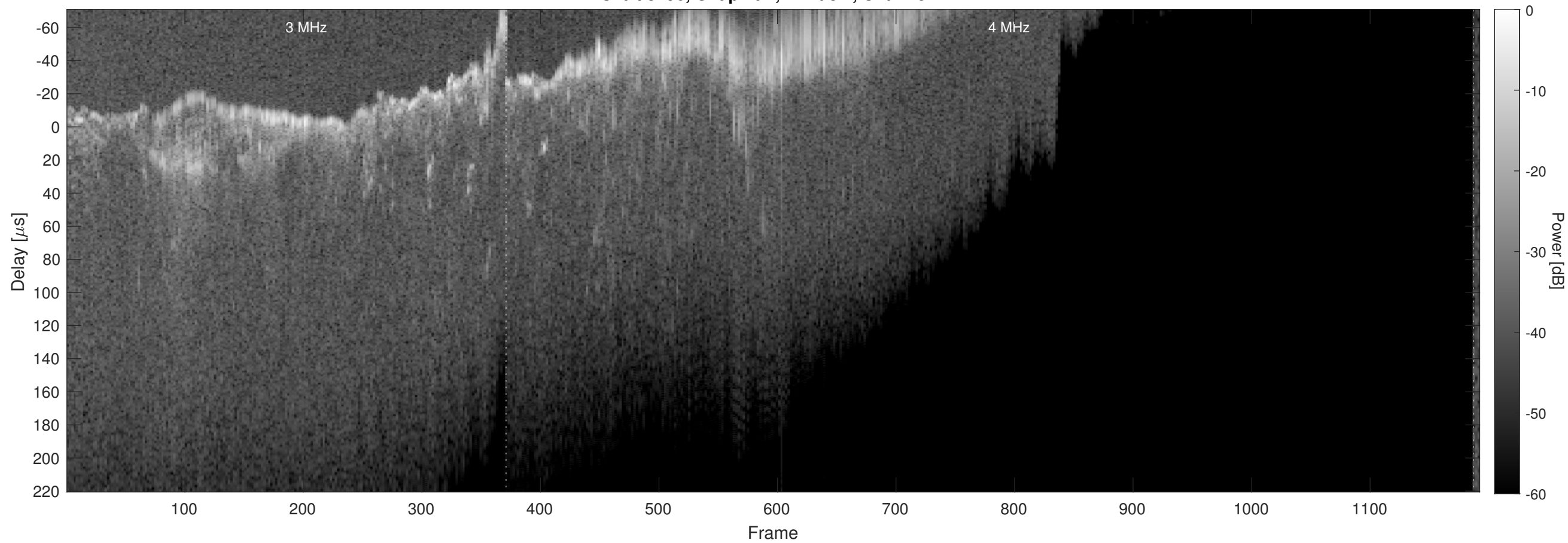
Orbit 8496, Chapman, Window, Channel 2
