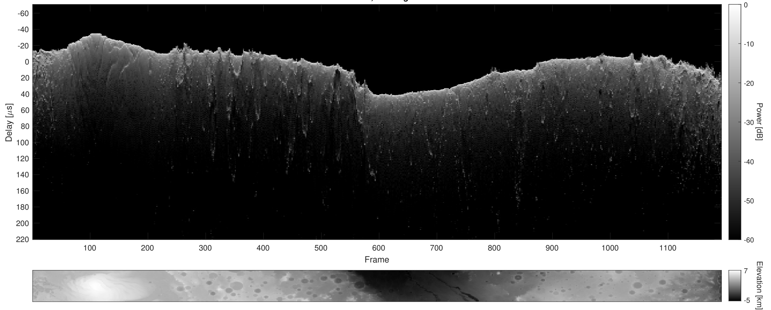
Orbit 8496, Cluttergram
