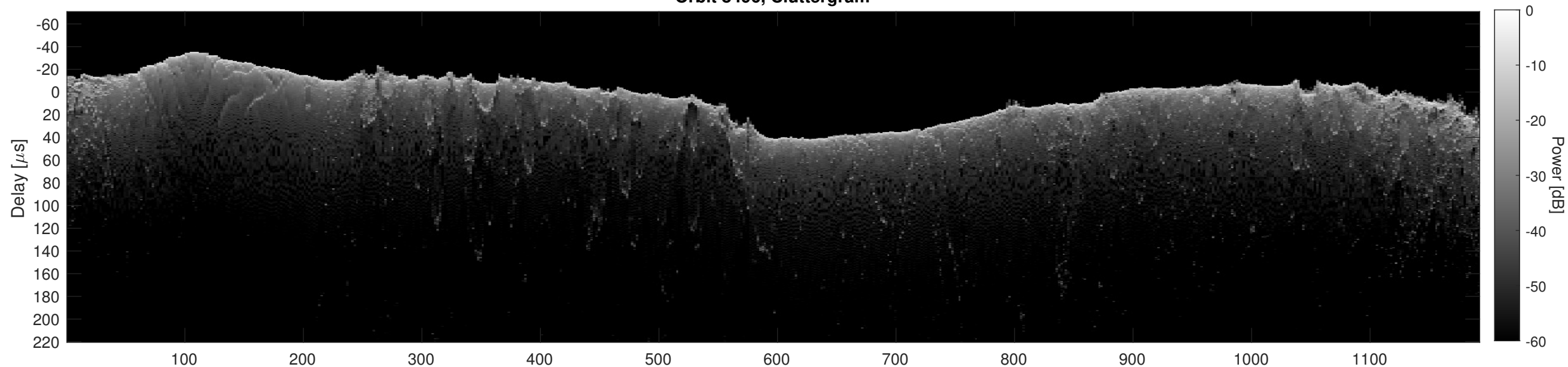
Orbit 8496, Cluttergram
