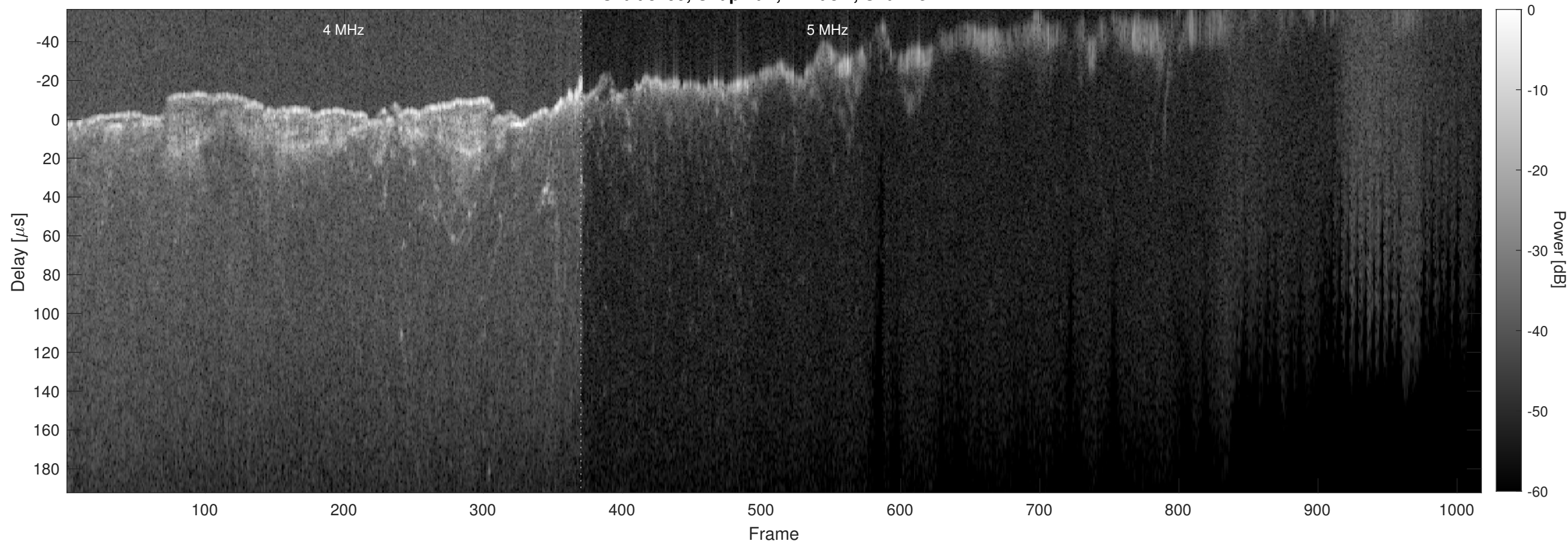
Orbit 8499, Chapman, Window, Channel 2
