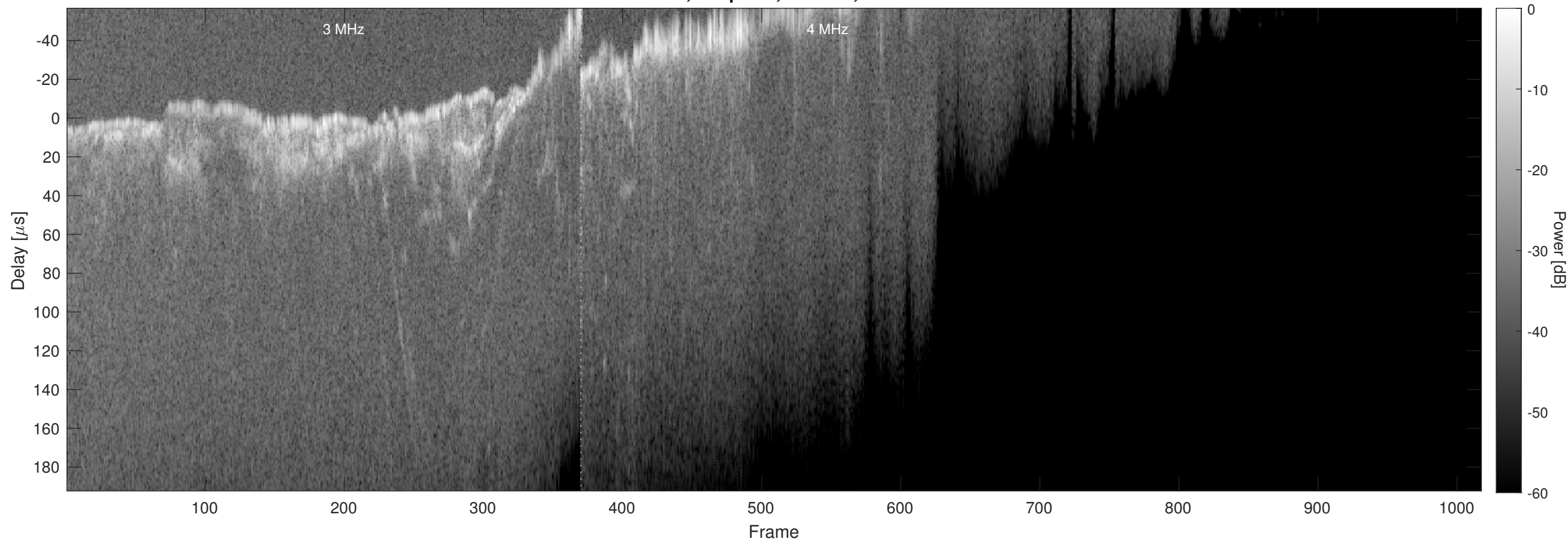
Orbit 8499, Chapman, Window, Channel 2
