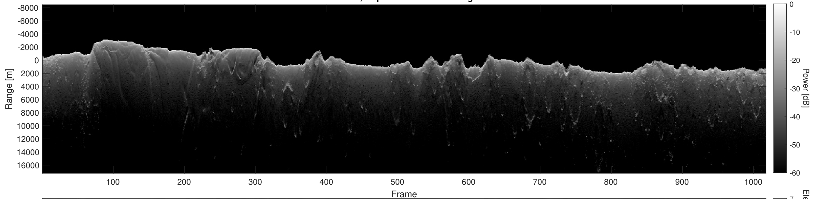
Orbit 8499, Depth-Corrected Cluttergram
