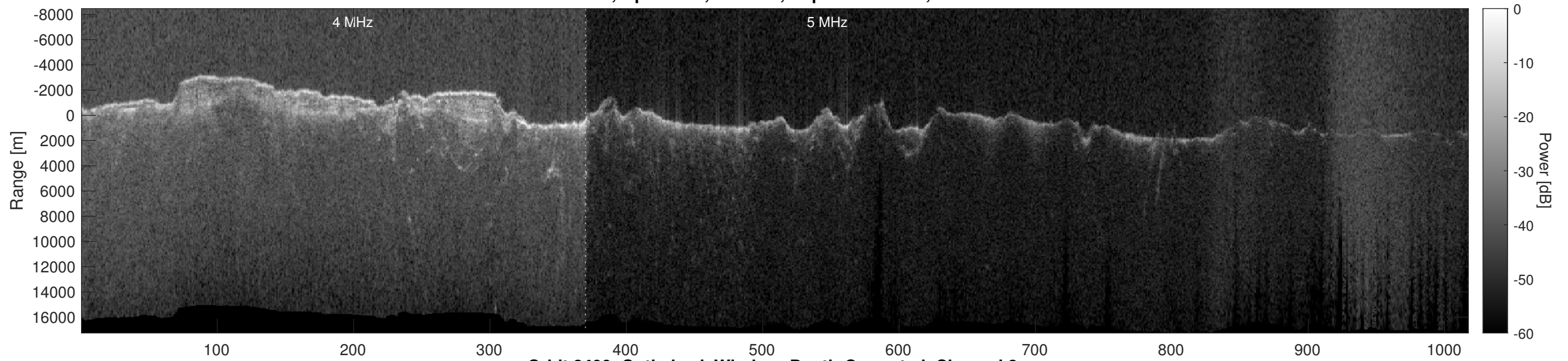
Orbit 8499, Optimized, Window, Depth-Corrected, Channel 2
