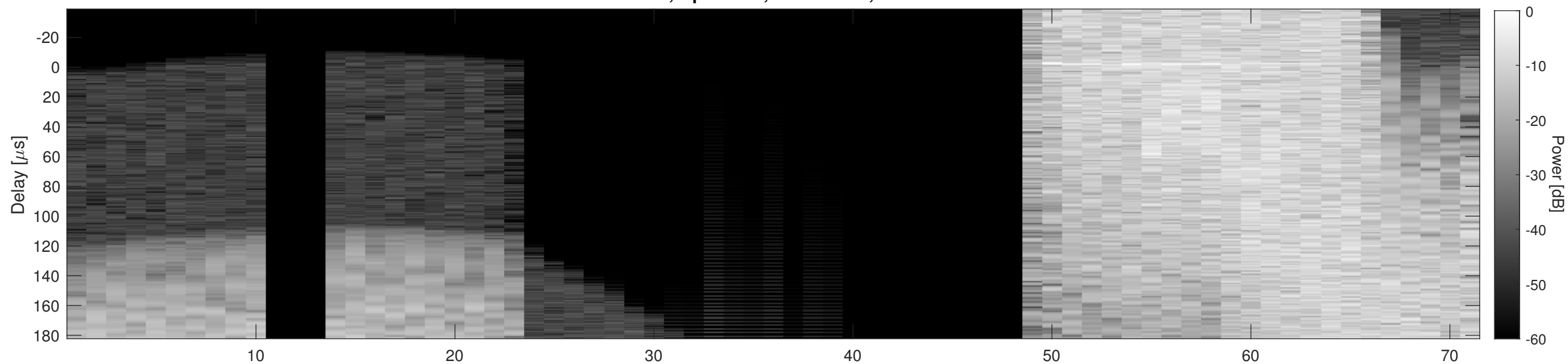
Orbit 8500, Cluttergram
