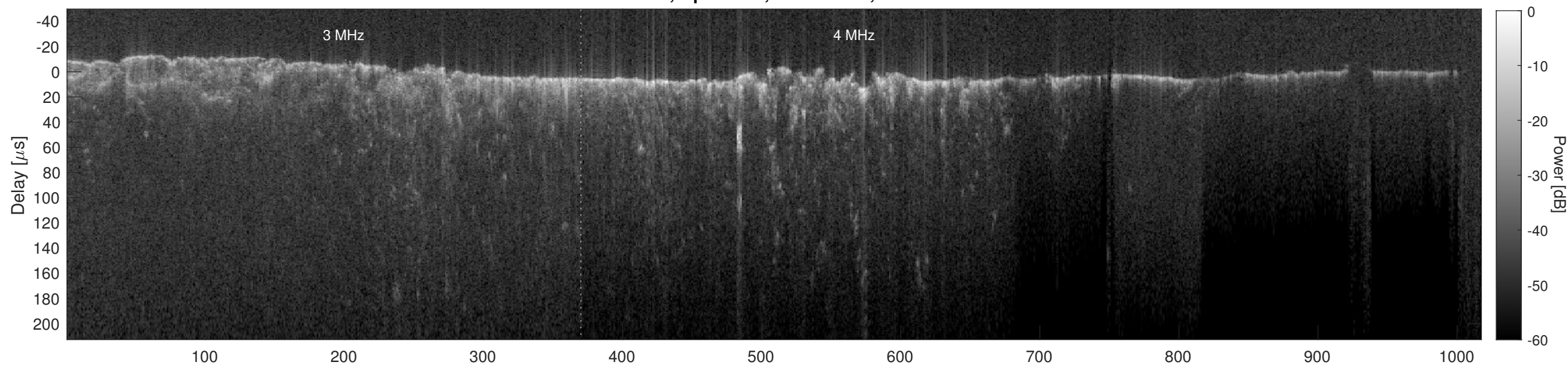
Orbit 8501, Cluttergram
