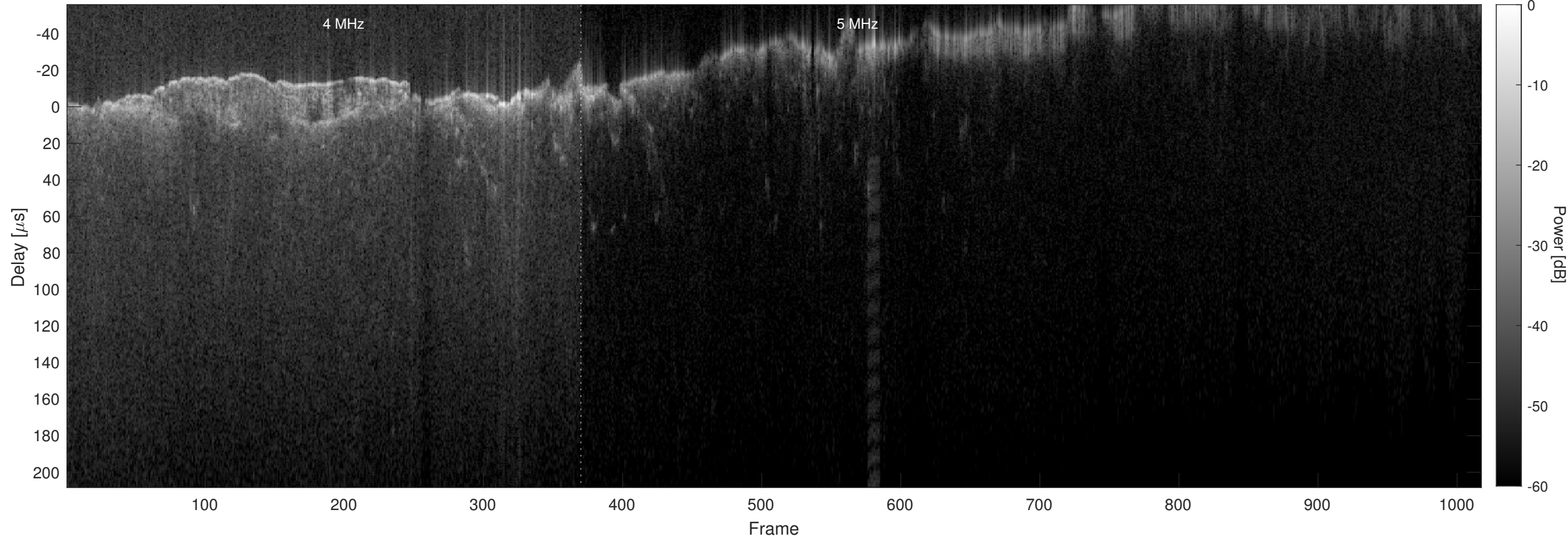
Orbit 8502, Chapman, No Window, Channel 2
