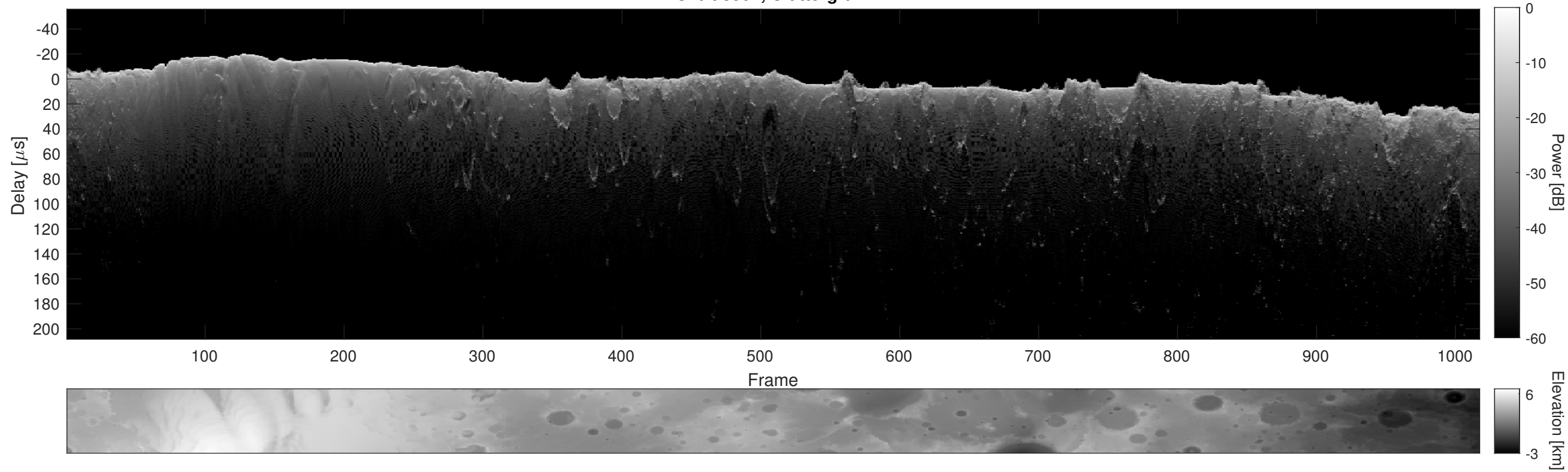
Orbit 8502, Cluttergram
