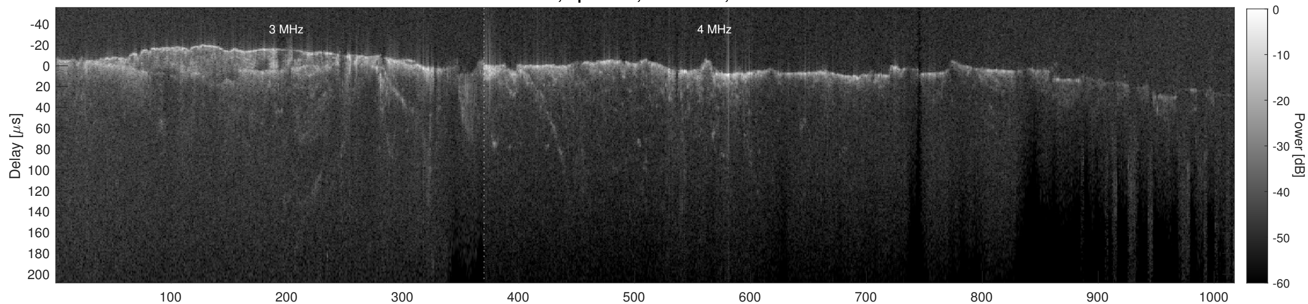
Orbit 8502, Cluttergram
