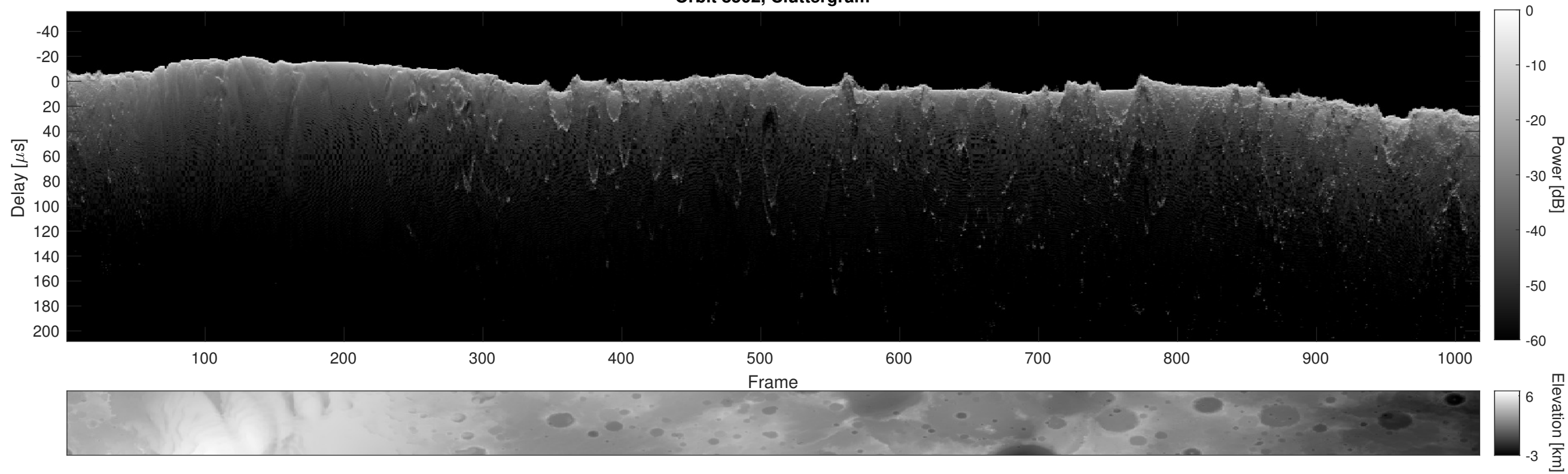
Orbit 8502, Cluttergram
