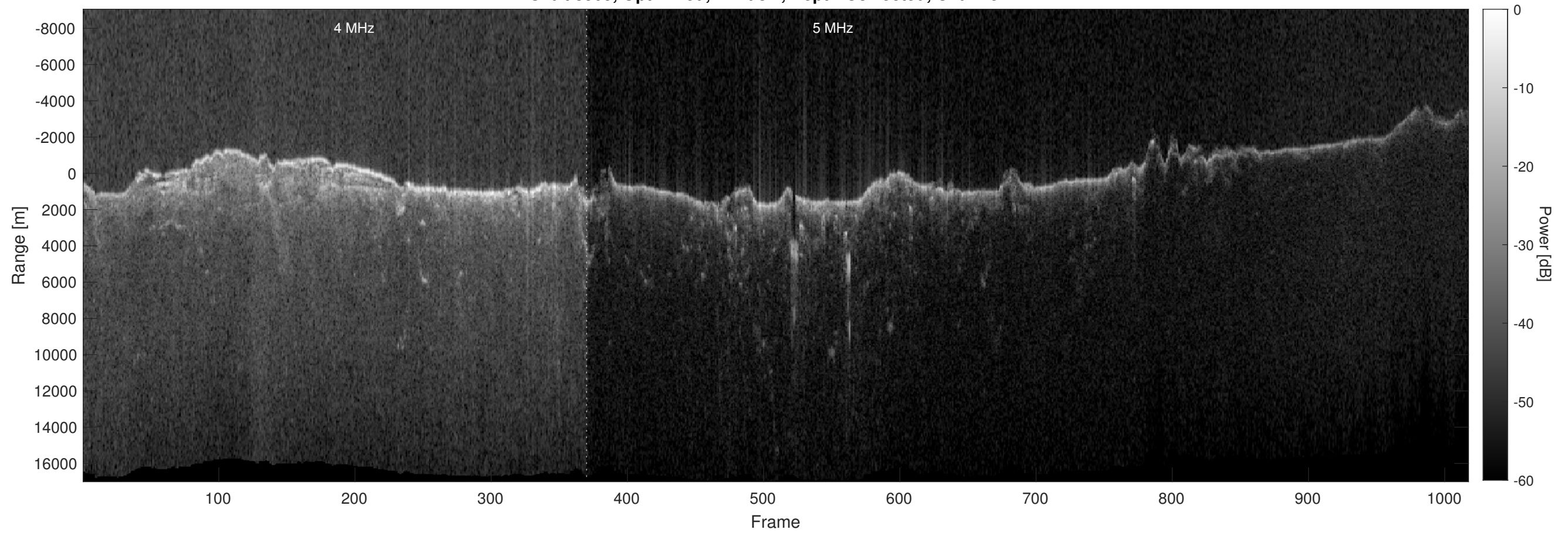
Orbit 8505, Optimized, Window, Depth-Corrected, Channel 2
