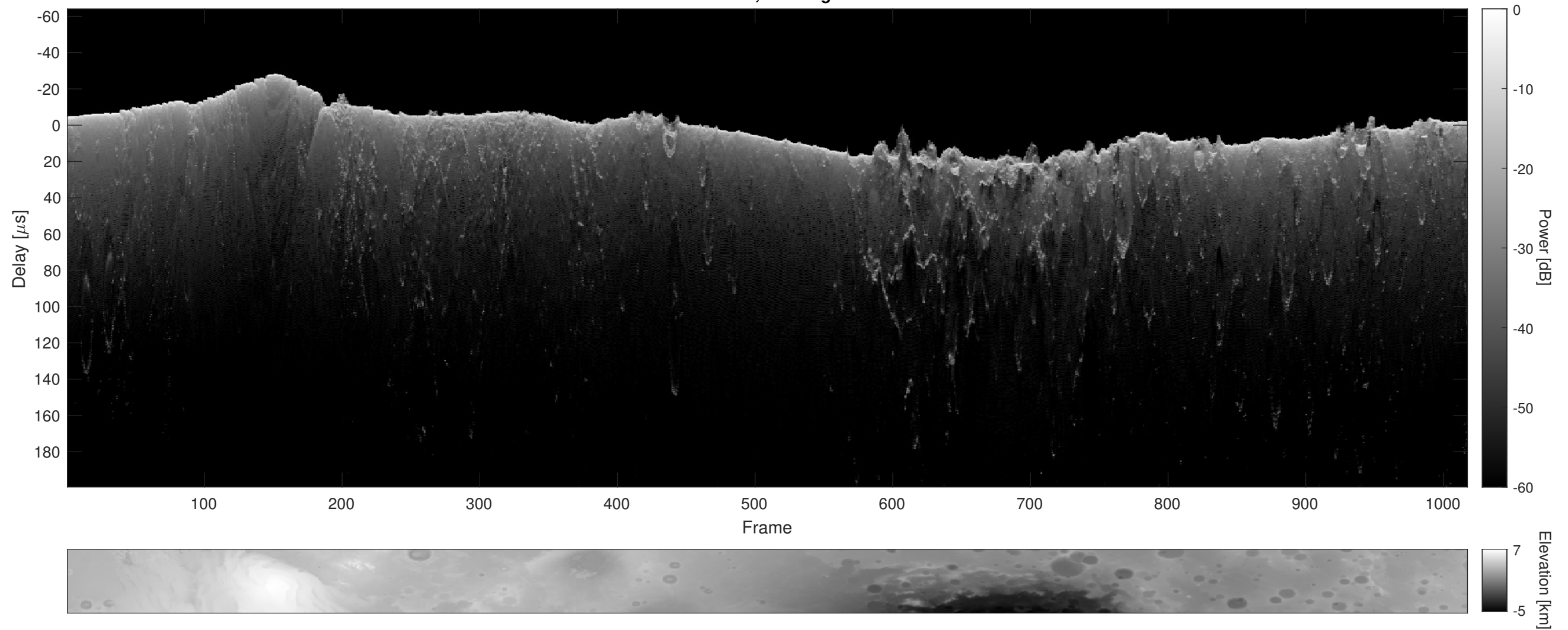
Orbit 8507, Cluttergram
