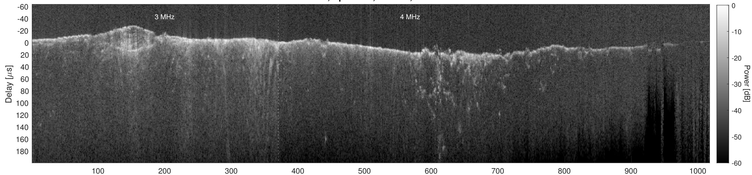
Orbit 8507, Cluttergram
