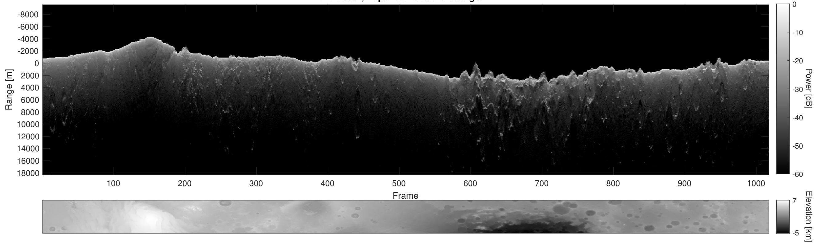
Orbit 8507, Depth-Corrected Cluttergram
