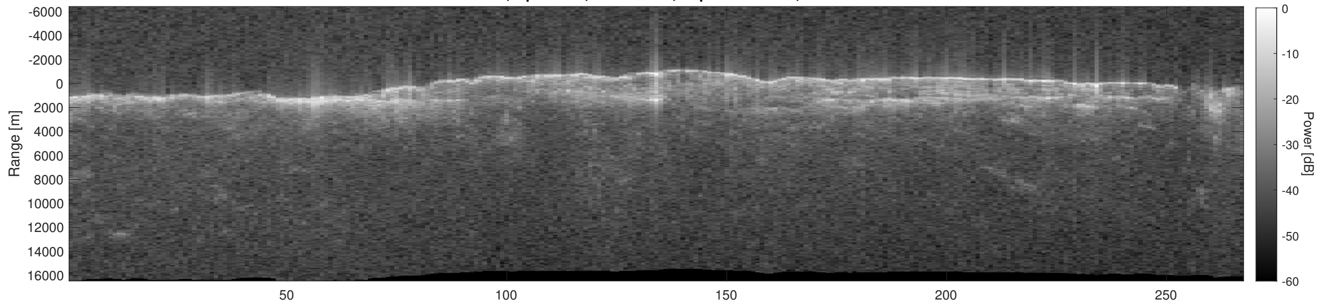
Orbit 8509, Depth-Corrected Cluttergram
