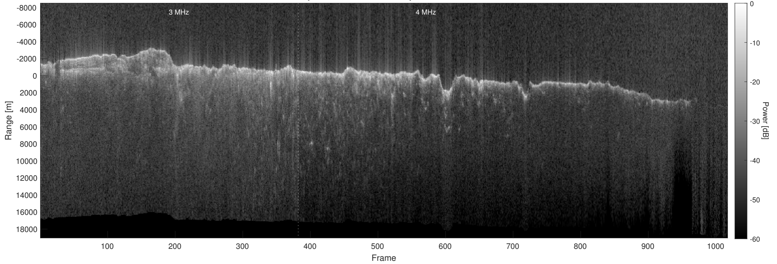
Orbit 8511, Optimized, No Window, Depth-Corrected, Channel 2
