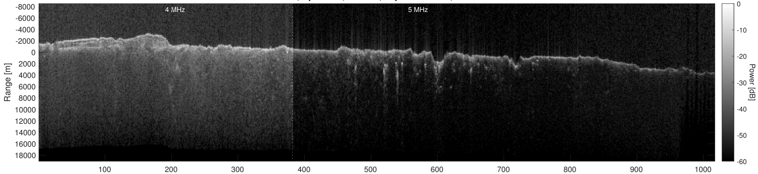
Orbit 8511, Optimized, Window, Depth-Corrected, Channel 2
