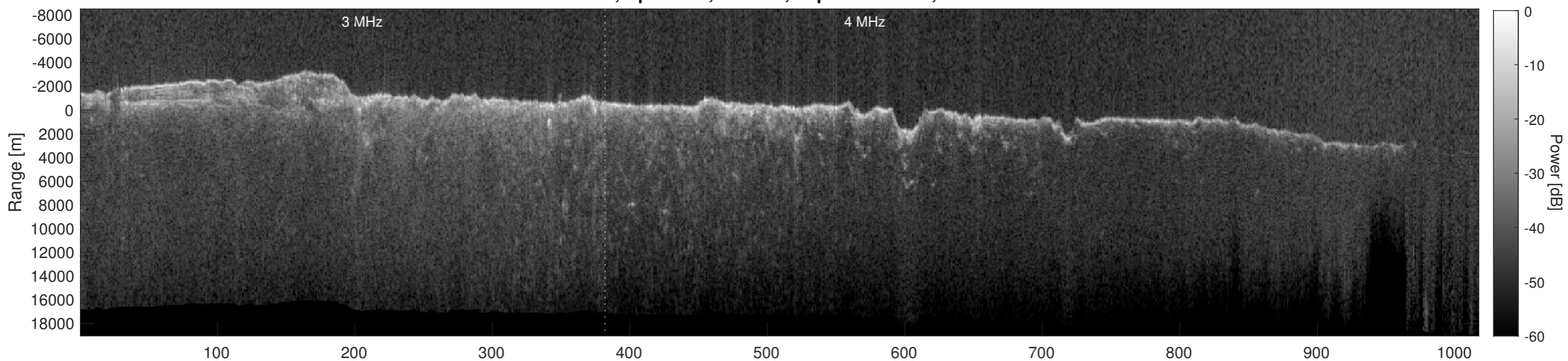
Orbit 8511, Depth-Corrected Cluttergram
