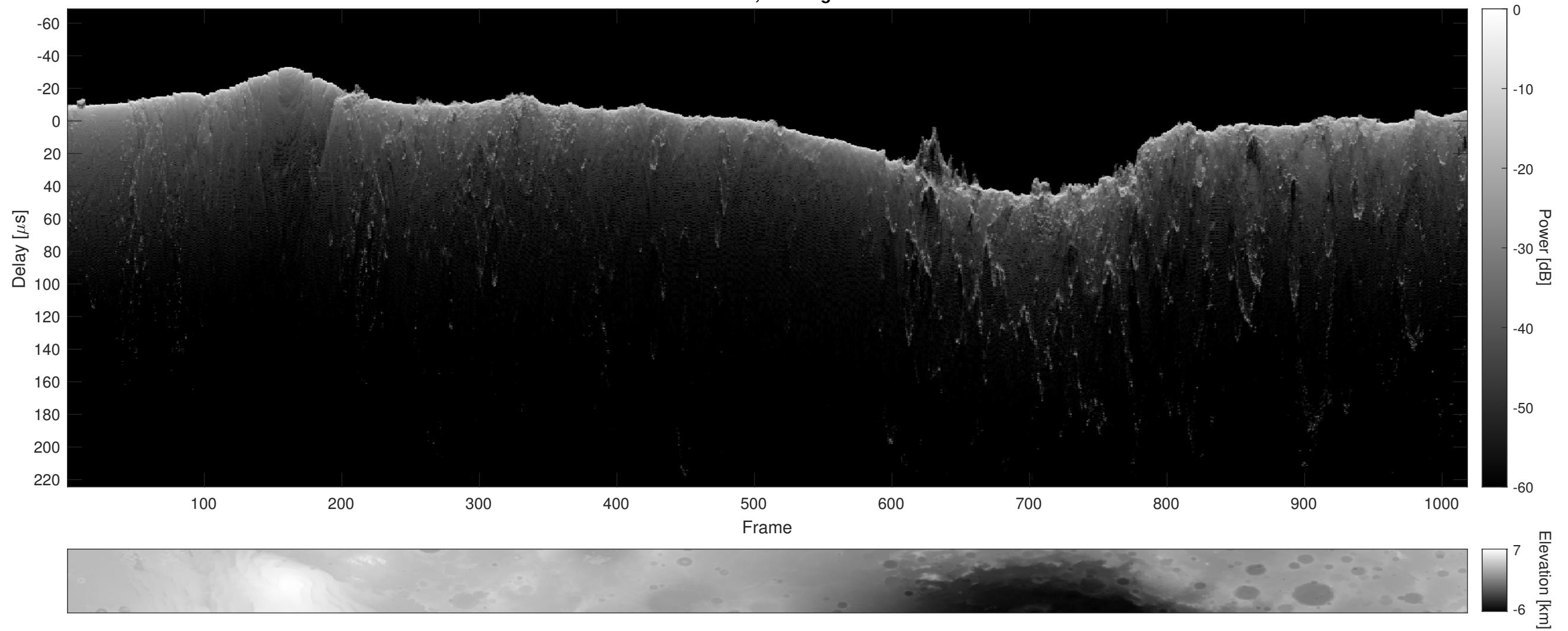
Orbit 8514, Cluttergram
