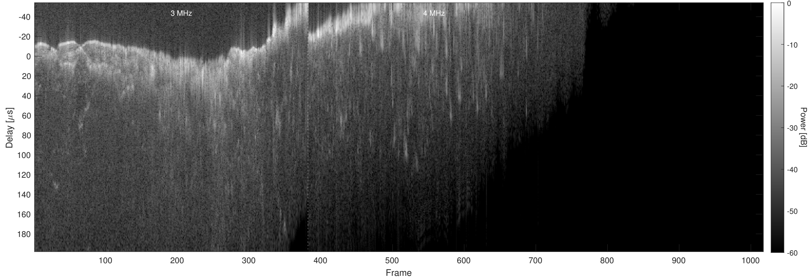
Orbit 8515, Chapman, No Window, Channel 2
