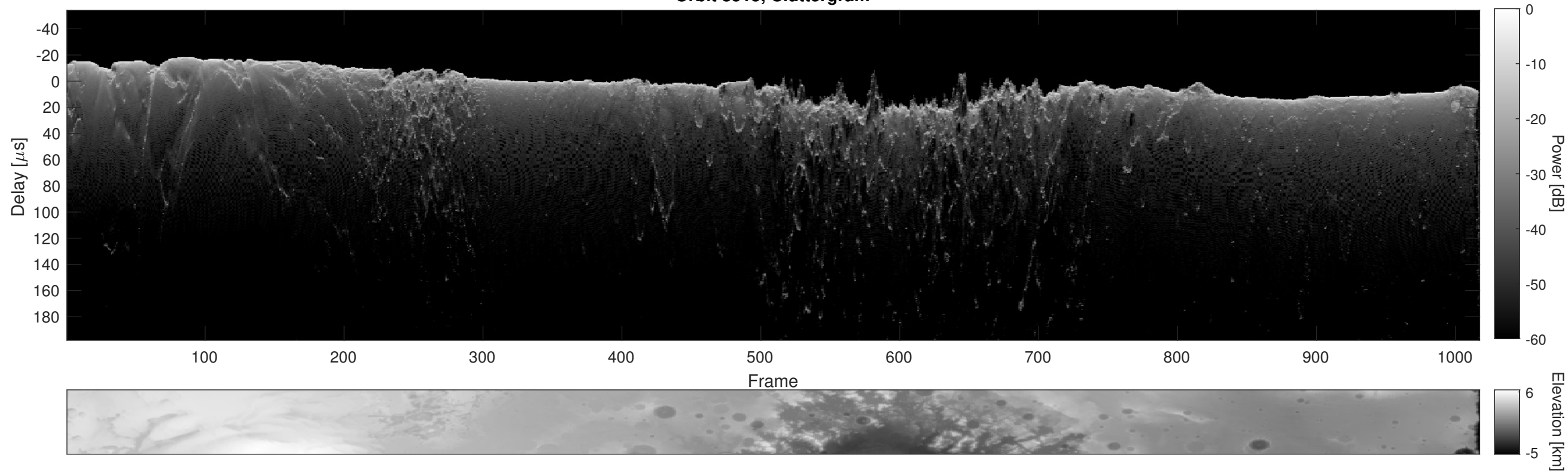
Orbit 8515, Cluttergram
