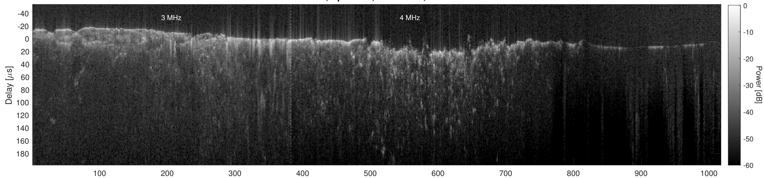
Orbit 8515, Cluttergram
