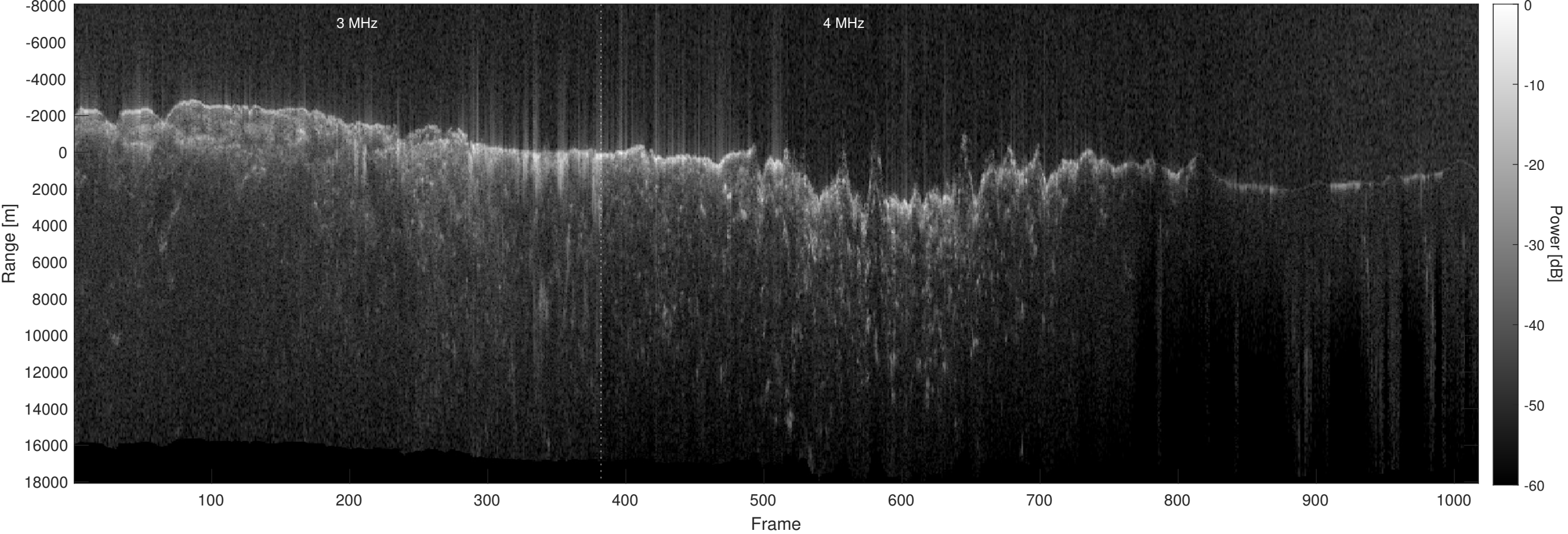
Orbit 8515, Optimized, No Window, Depth-Corrected, Channel 2
