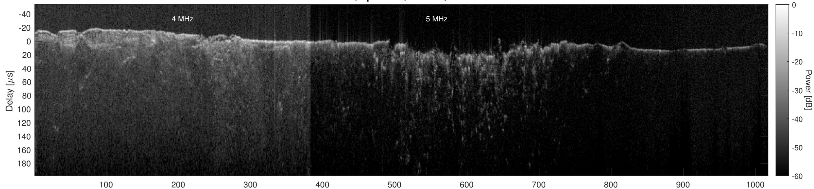
Orbit 8515, Optimized, Window, Channel 2
