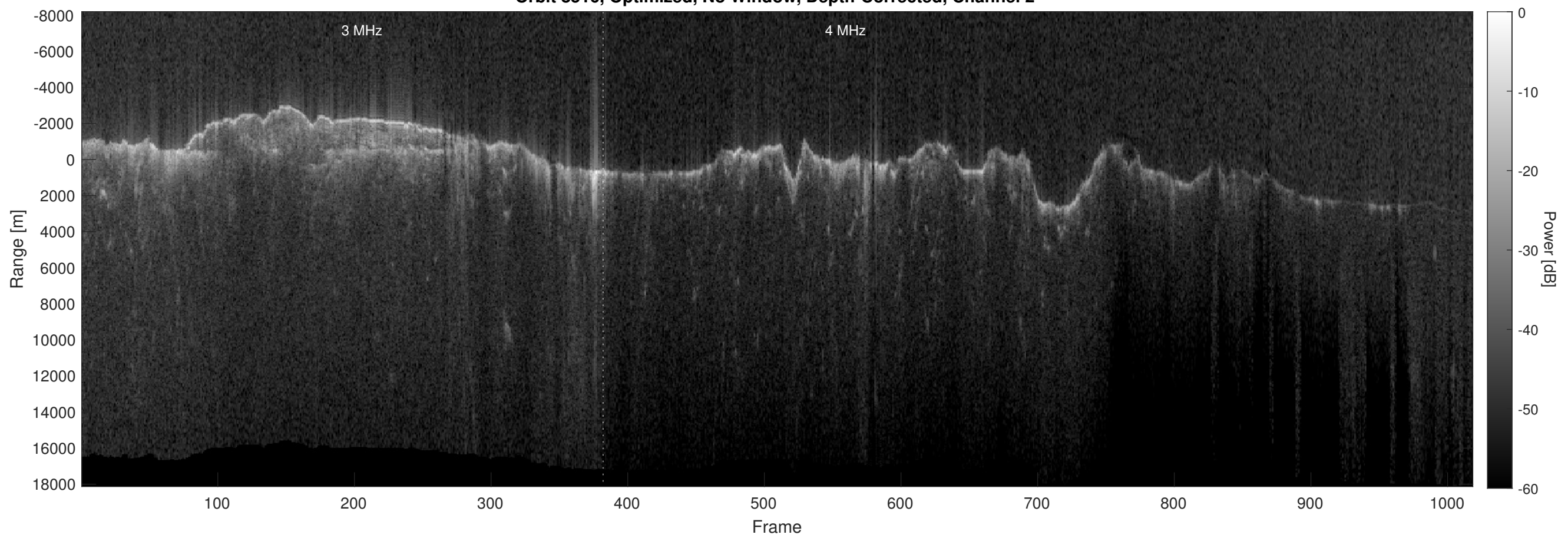
Orbit 8516, Optimized, No Window, Depth-Corrected, Channel 2
