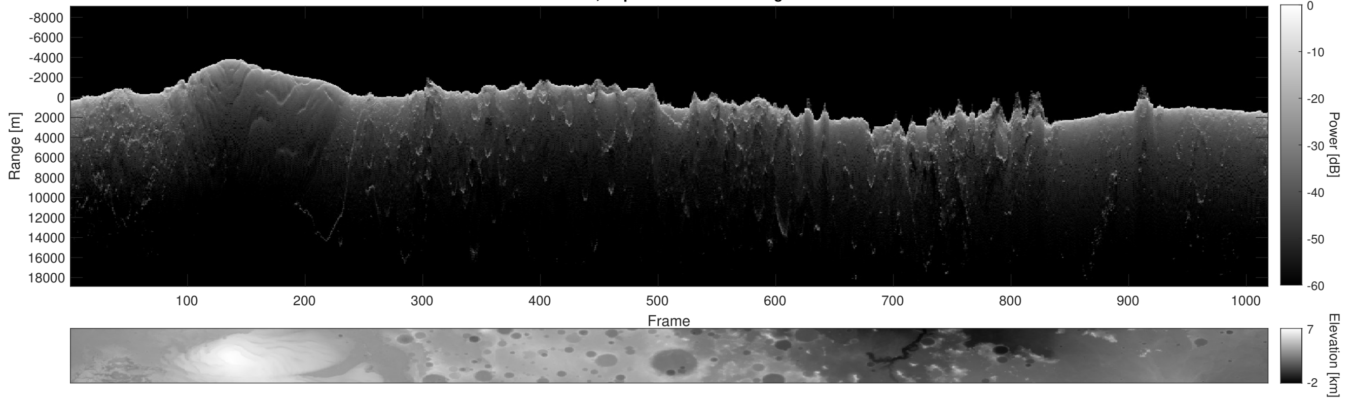
Orbit 8517, Depth-Corrected Cluttergram
