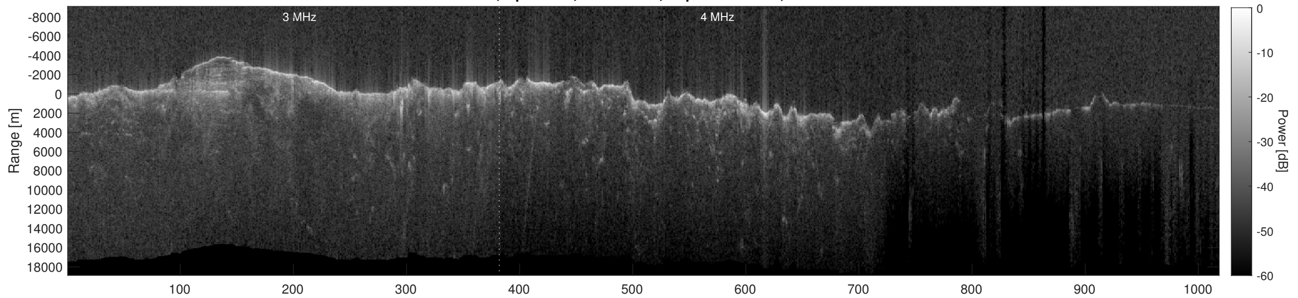
Orbit 8517, Depth-Corrected Cluttergram
