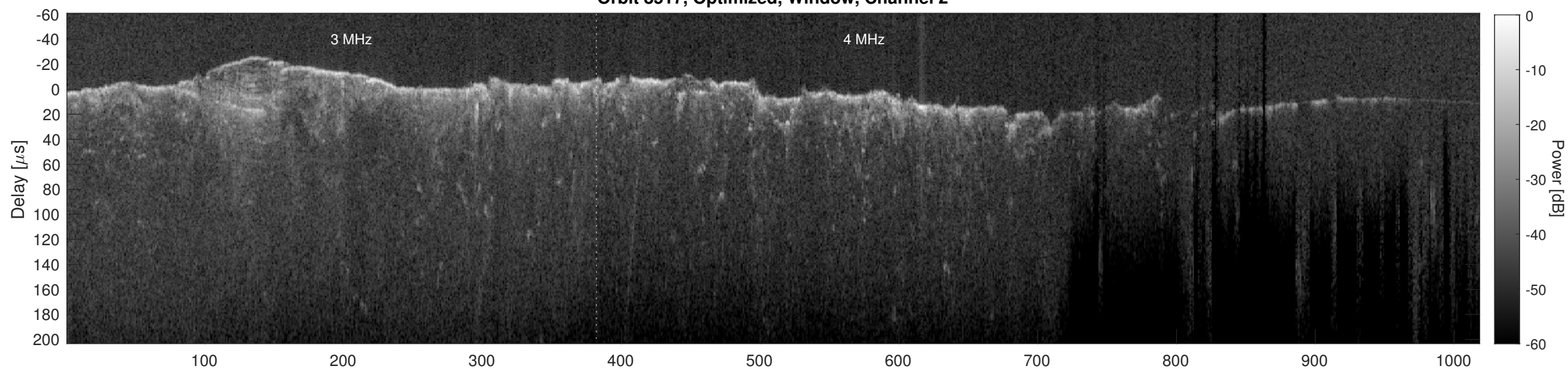
Orbit 8517, Cluttergram
