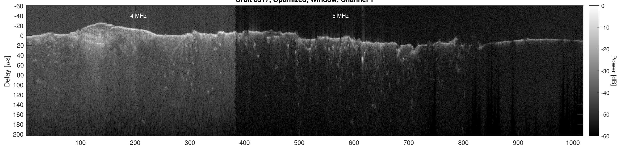
Orbit 8517, Optimized, Window, Channel 2
