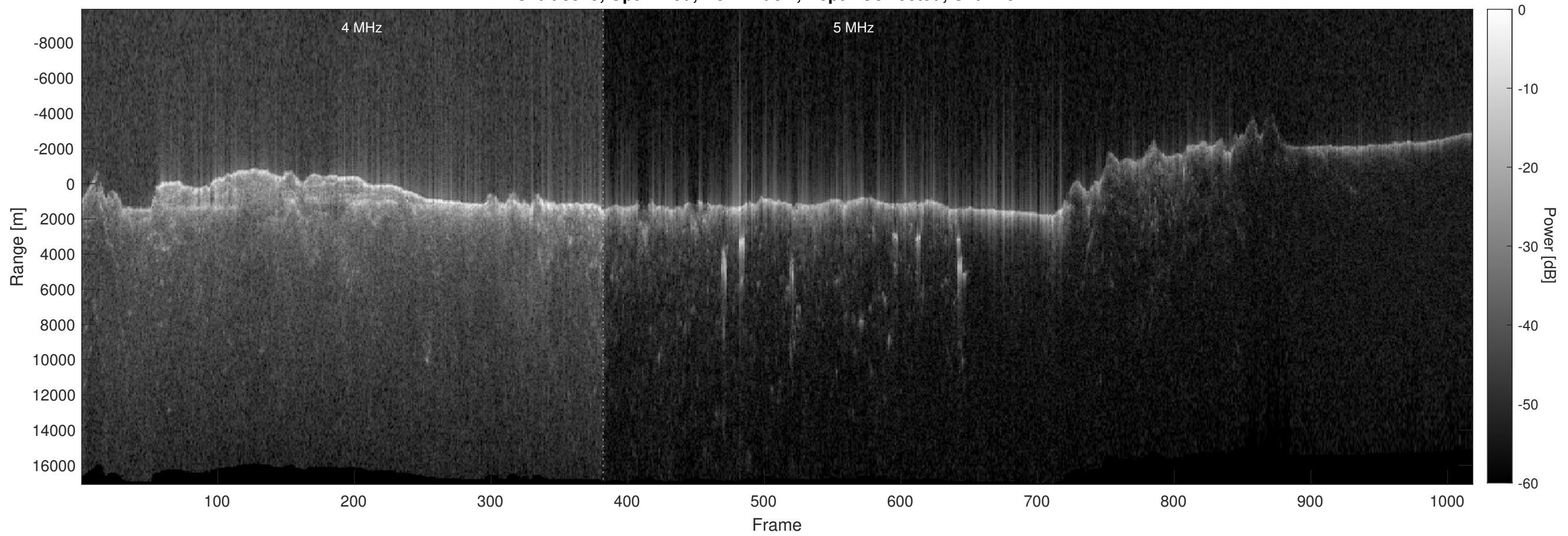
Orbit 8519, Optimized, No Window, Depth-Corrected, Channel 2
