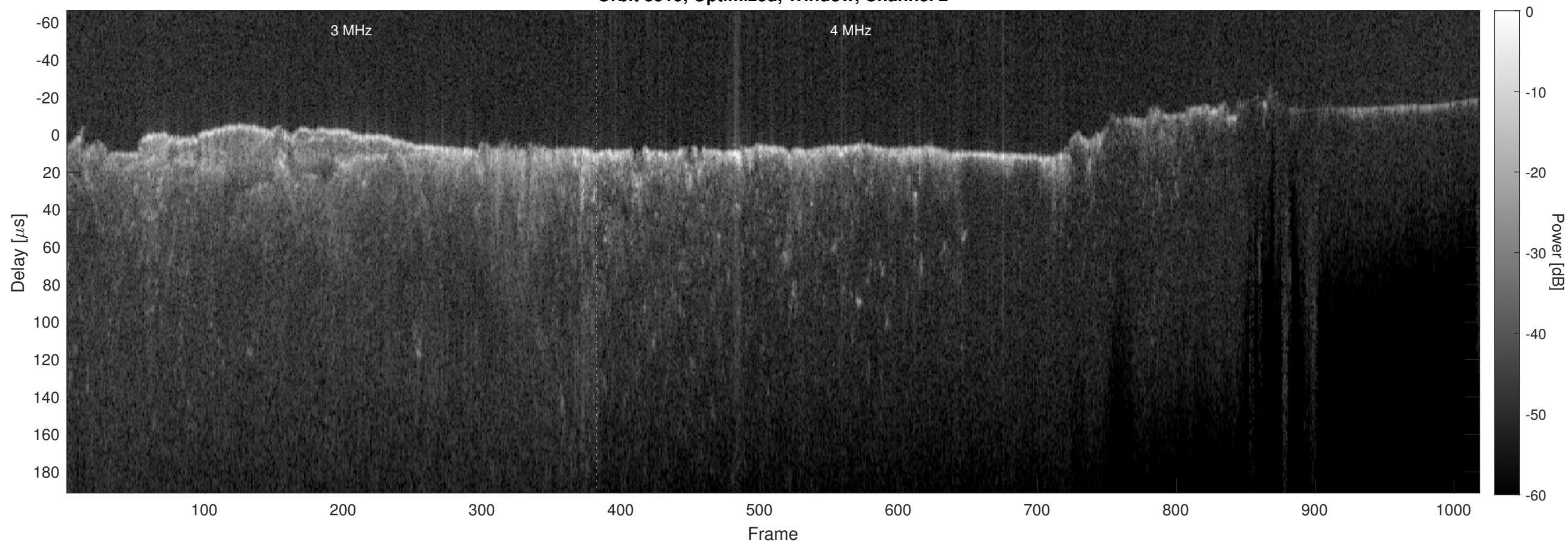
Orbit 8519, Optimized, Window, Channel 2
