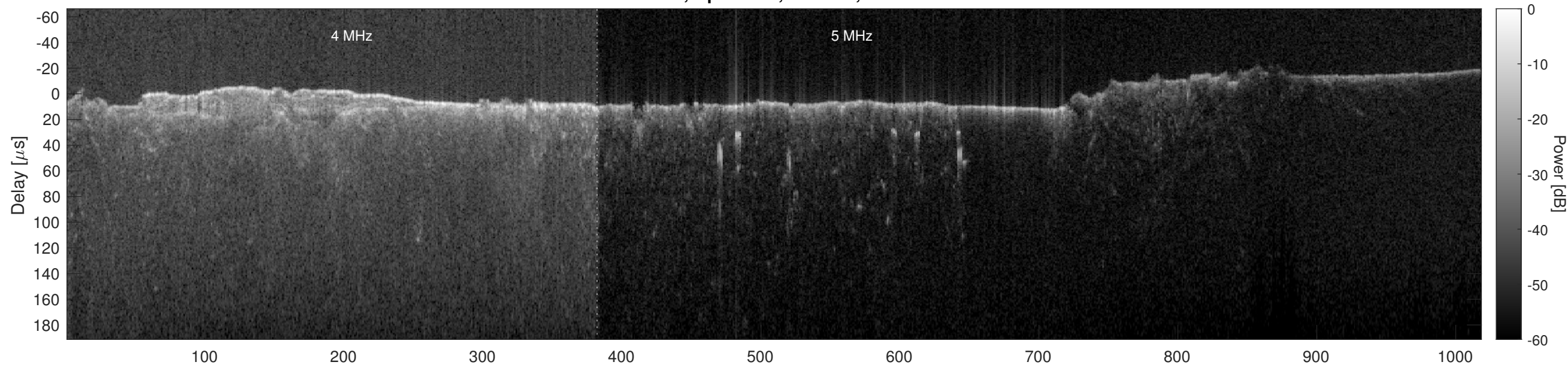
Orbit 8519, Optimized, Window, Channel 2
