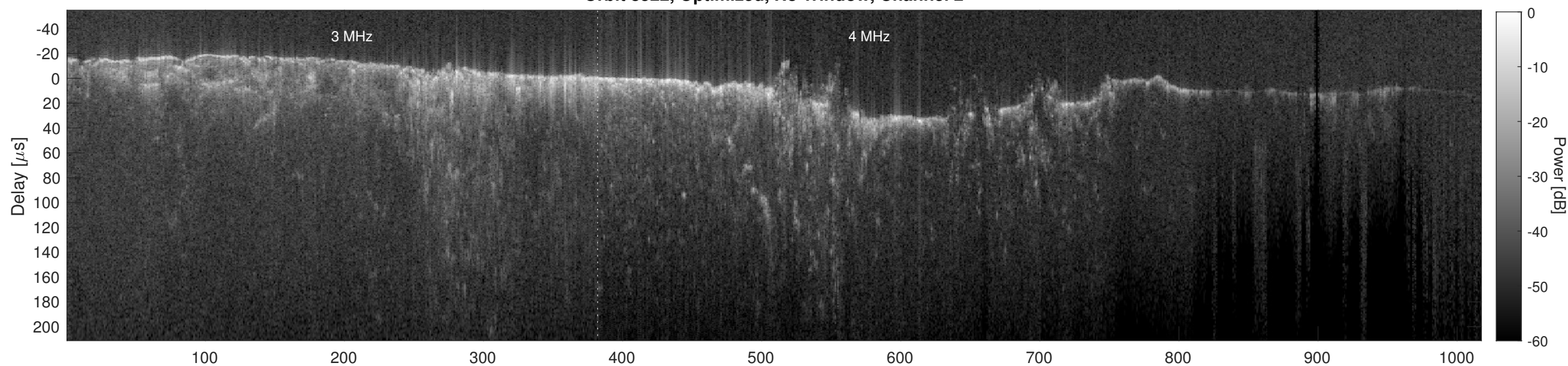
Orbit 8522, Cluttergram
