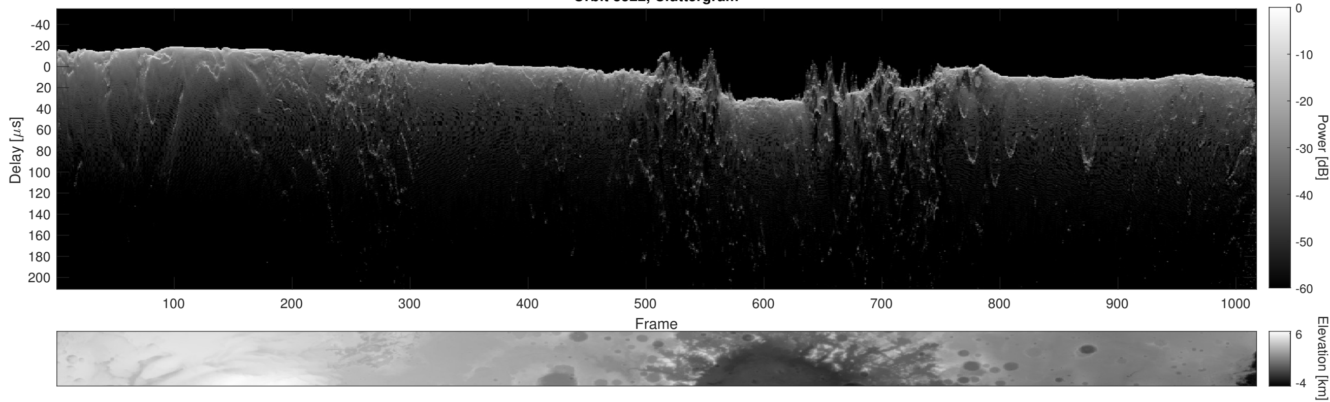
Orbit 8522, Cluttergram
