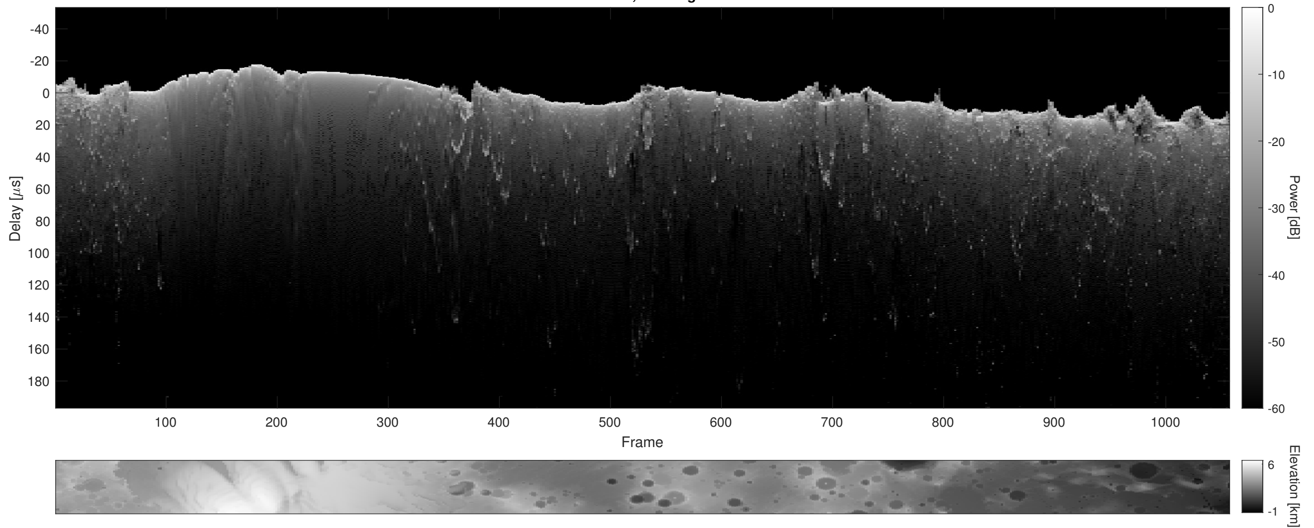
Orbit 8523, Cluttergram
