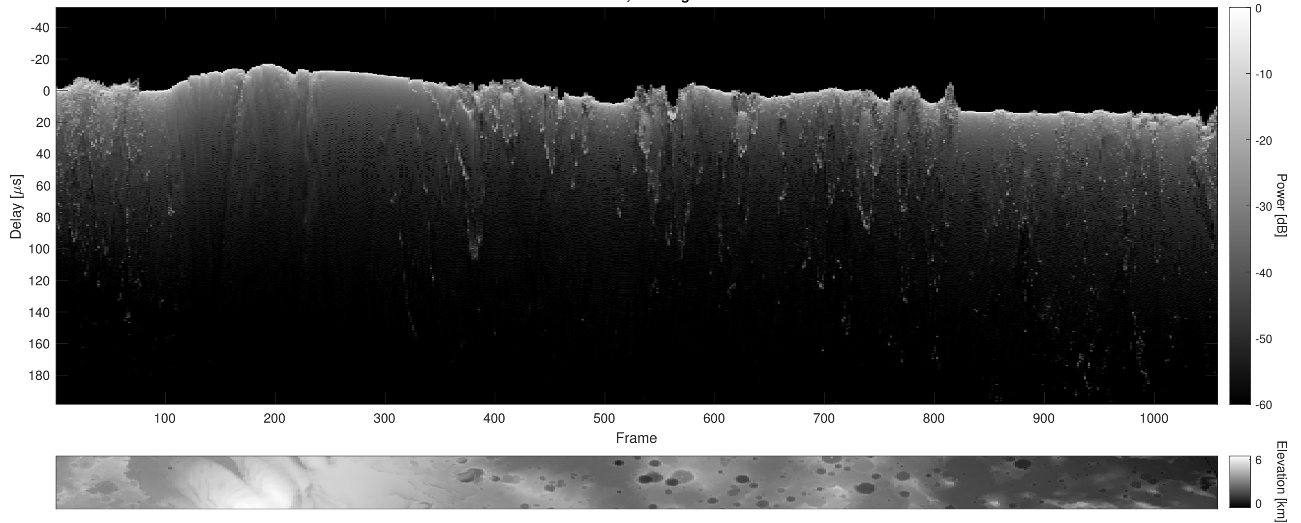
Orbit 8530, Cluttergram
