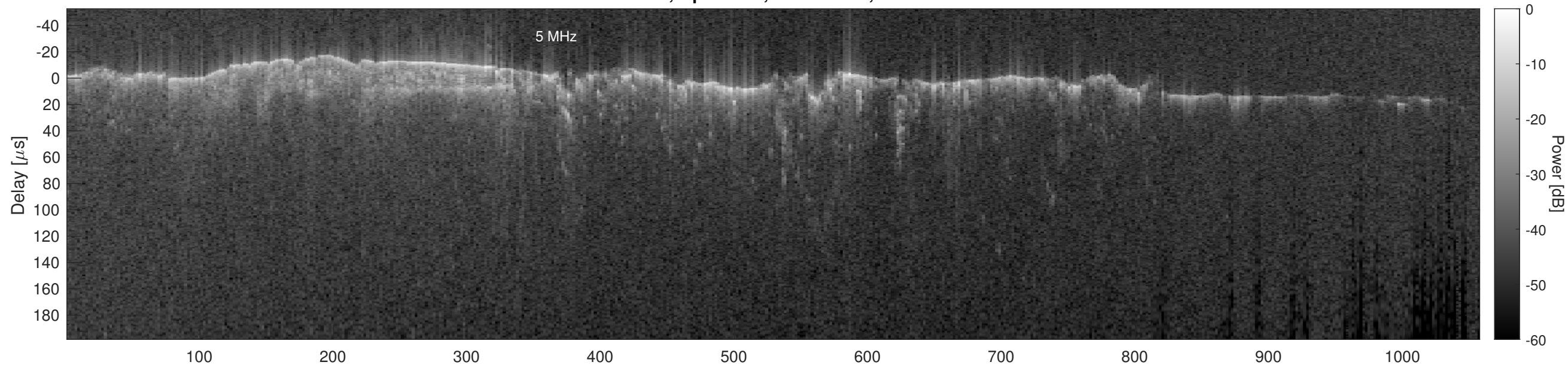
Orbit 8530, Optimized, No Window, Channel 2
