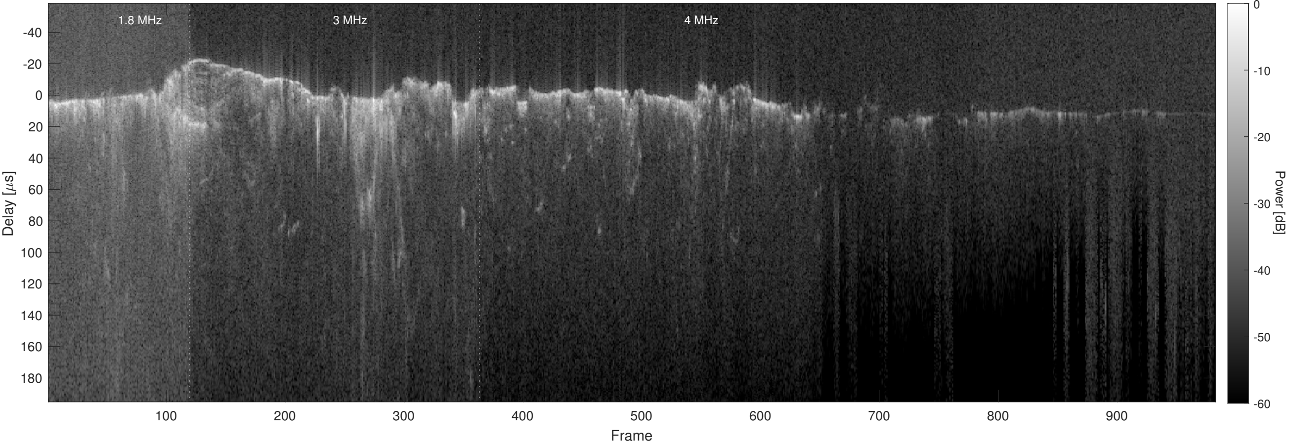
Orbit 8531, Optimized, No Window, Channel 2
