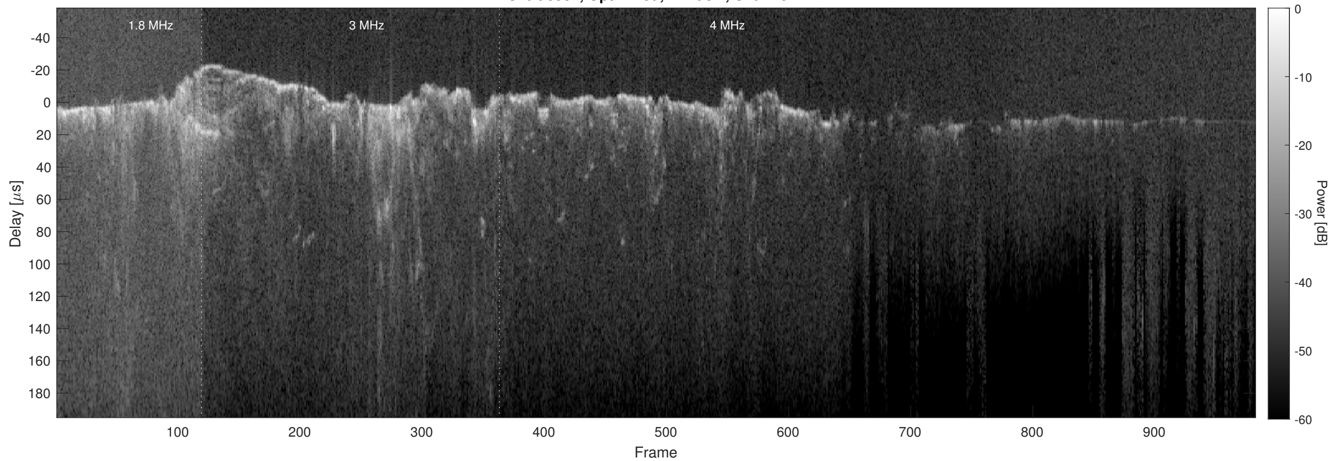
Orbit 8531, Optimized, Window, Channel 2
