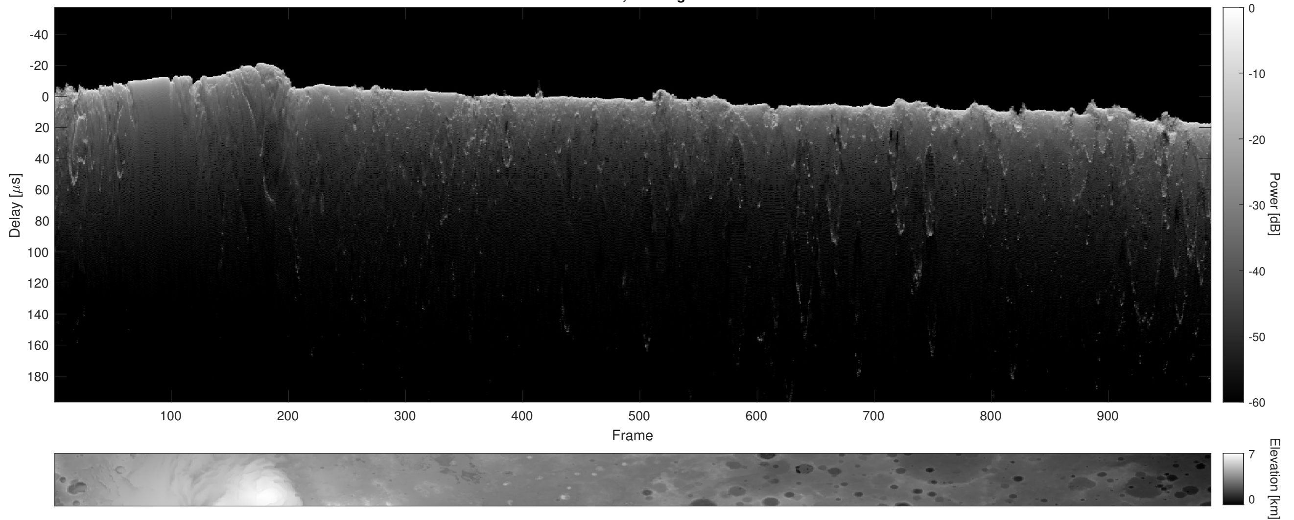
Orbit 8532, Cluttergram
