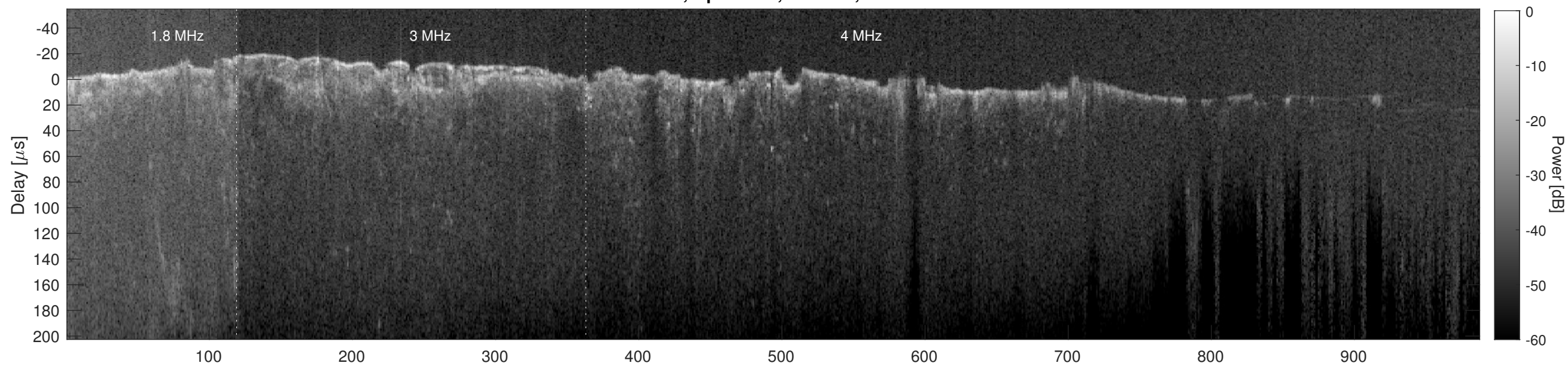
Orbit 8534, Cluttergram
