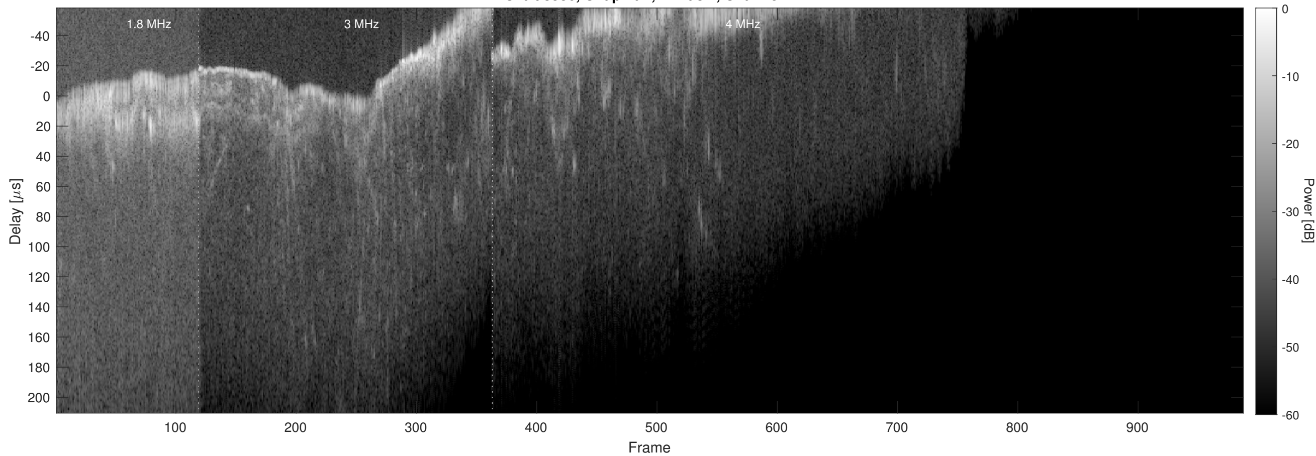
Orbit 8536, Chapman, Window, Channel 2
