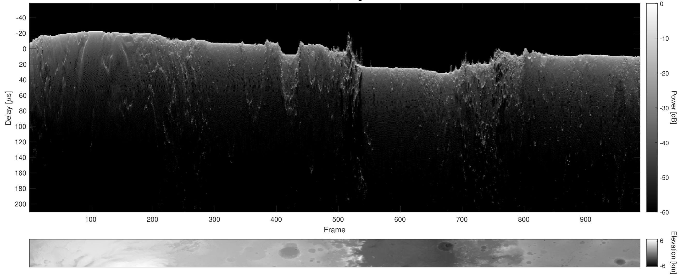
Orbit 8536, Cluttergram
