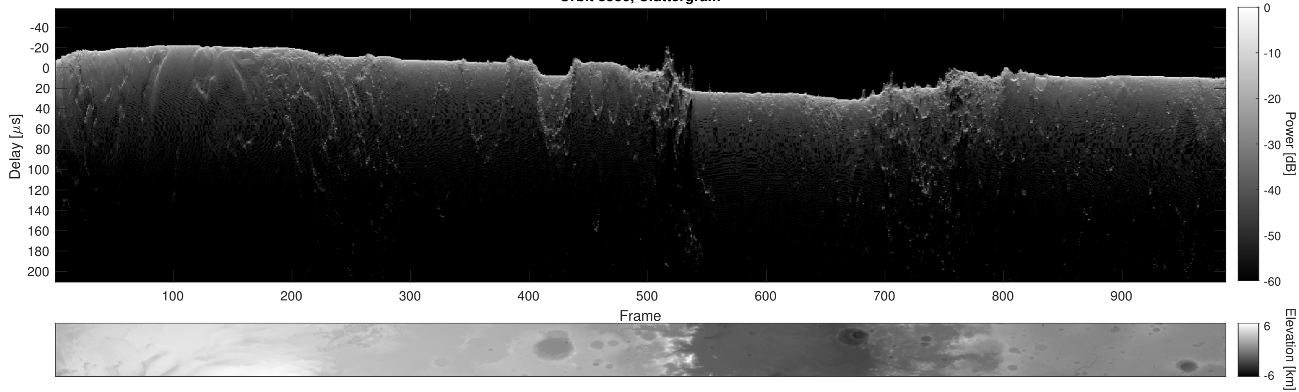
Orbit 8536, Cluttergram
