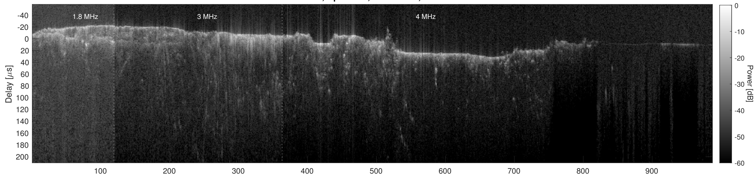
Orbit 8536, Cluttergram
