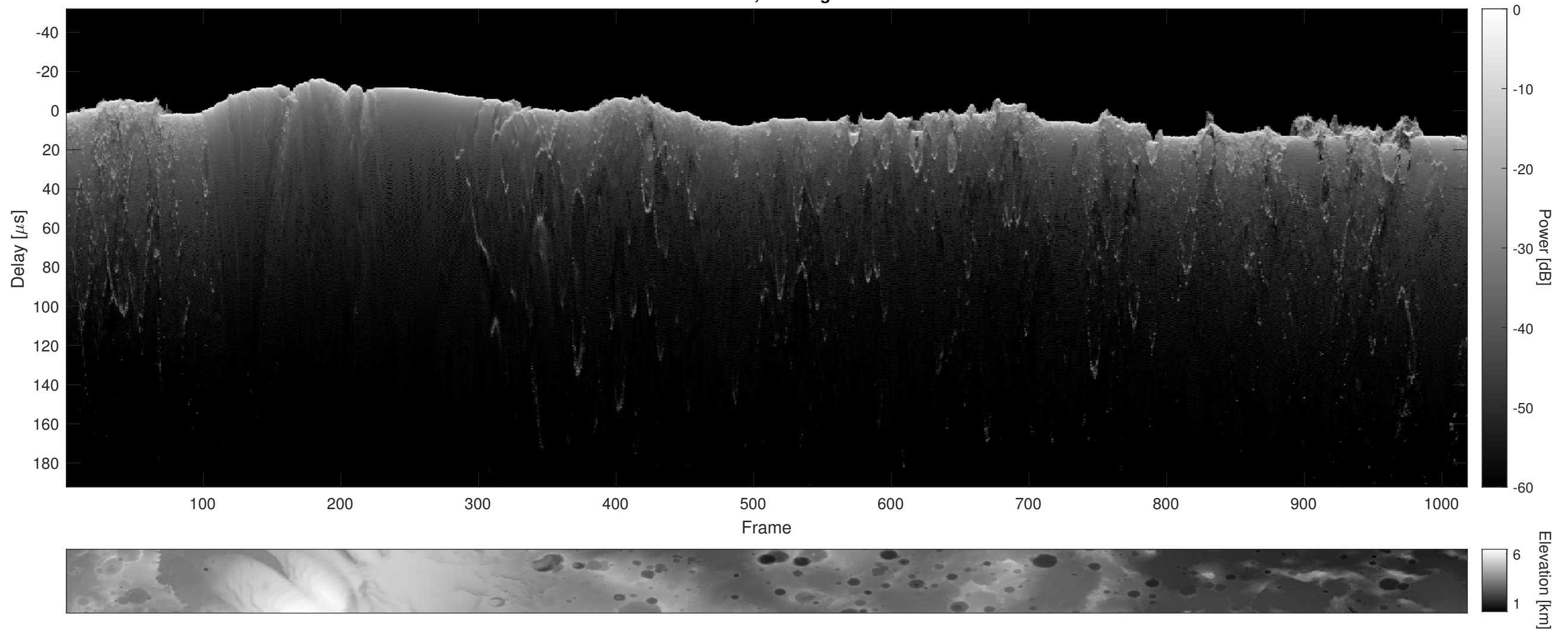
Orbit 8537, Cluttergram
