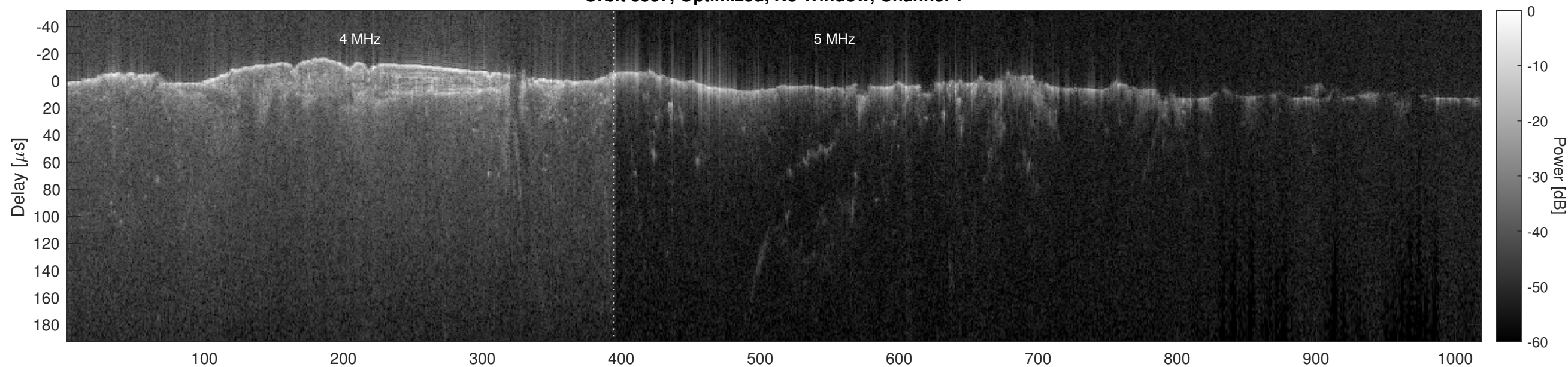
Orbit 8537, Optimized, No Window, Channel 2
