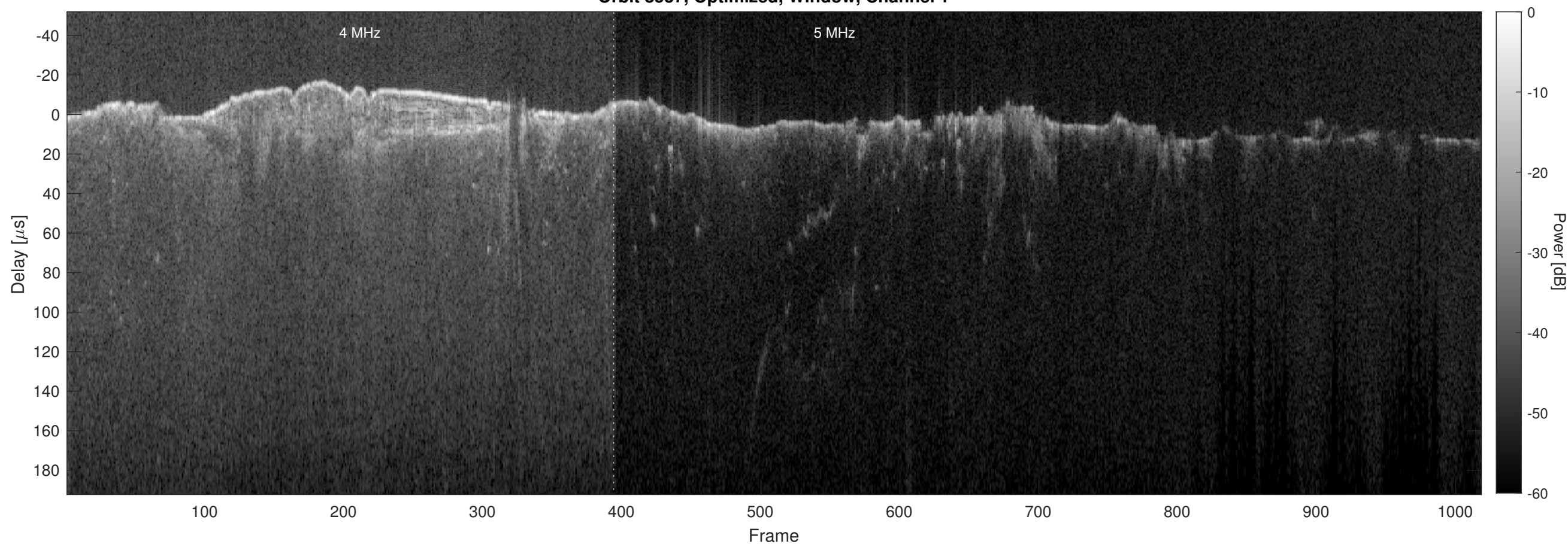
Orbit 8537, Optimized, Window, Channel 2
