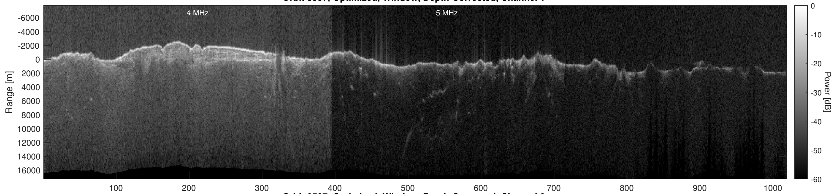
Orbit 8537, Optimized, Window, Depth-Corrected, Channel 2
