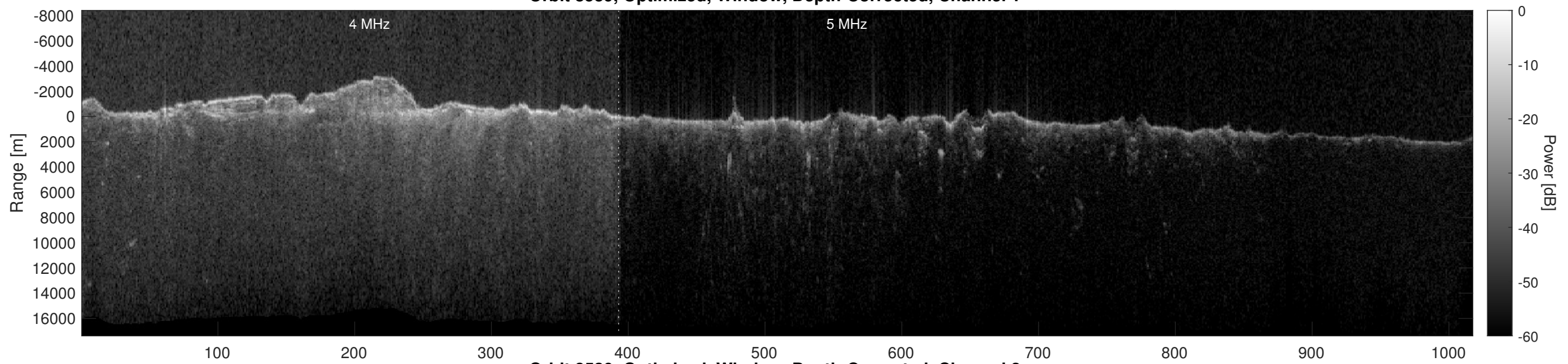
Orbit 8539, Optimized, Window, Depth-Corrected, Channel 2
